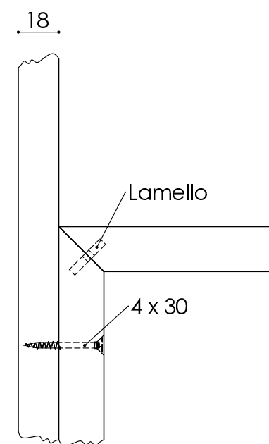
DETAIL E
